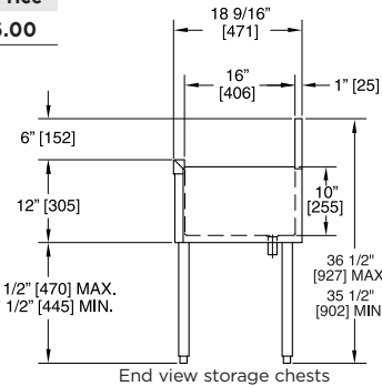
End view storage chests
