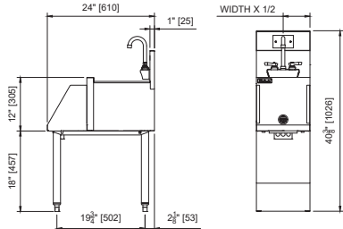
End view blender station with sink
