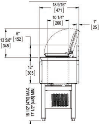
End view ice cream cabinet
