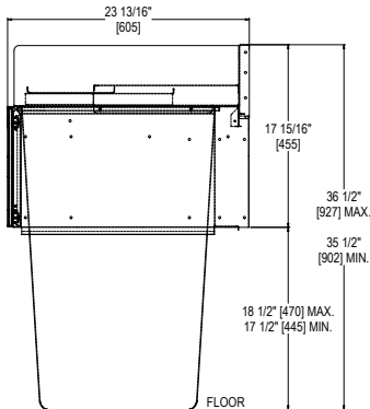
End view trash receptacle
