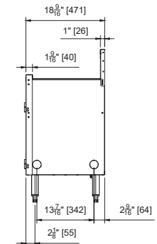
End view storage cabinet with sink
