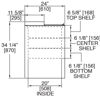
End view for 2' model
