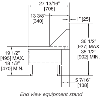
End view equipment stand
