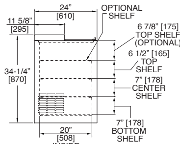
End view for 3', 4', & 5' models
