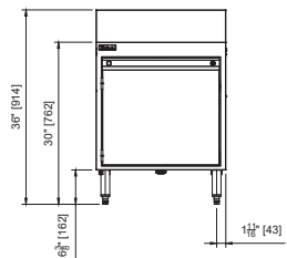
Front view storage bin
