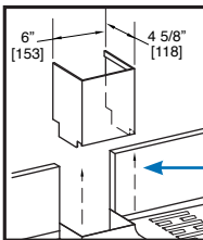
TS6CO-BW (with 7055-66 backsplash chase)
