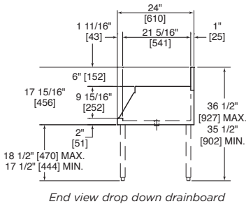
End view drop down drainboard
