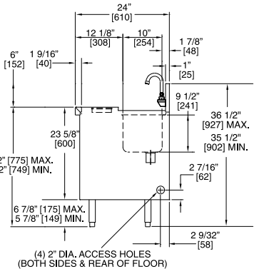
End View Storage Cabinet with Sink
