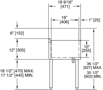
End view storage chests
