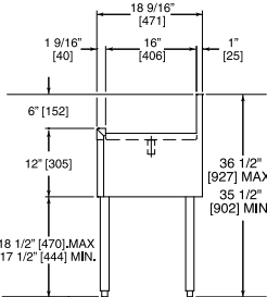
TS end view drainboard
