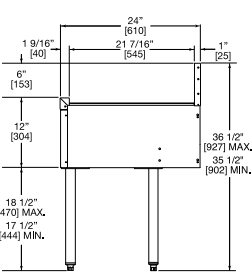
TSF end view drainboard
