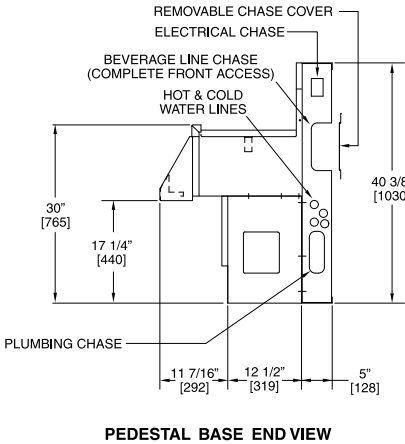
Typical modular bar section (Underbar equipment not shown. Order separately)
