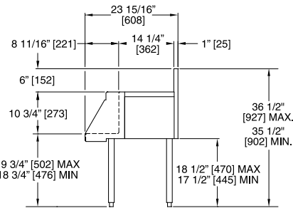
End view blender station with flat work surface
