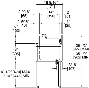
End view sink module
