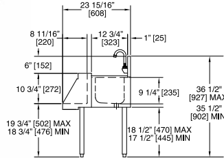
End view blender station with sink
