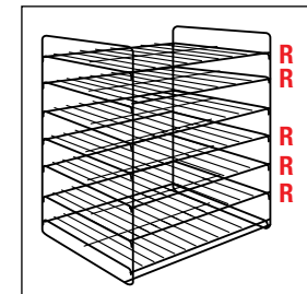
7-Shelf Multi-Purpose Rack FSDT7SMP (Max. 18" x 13" Half-Size Sheet Pans) (2 1/2" between shelves)
